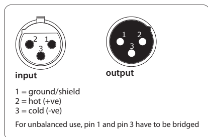
Fig. 5.1: XLR connections
