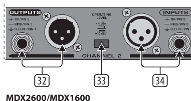
Fig. 2.8: Rear panel connectors and switches
