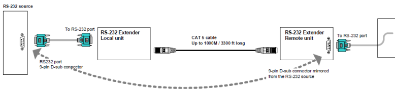
Figure 1: RS-232 Extender Connection Diagram
