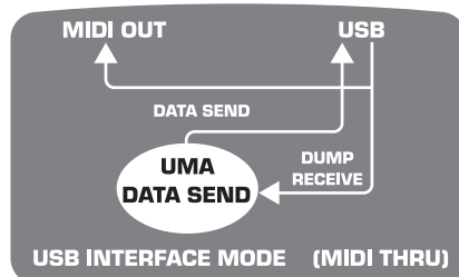
Fig. 1.5: USB mode with MIDI THRU
