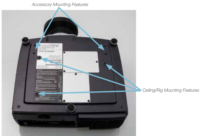
Figure 5-13. Mounting features
