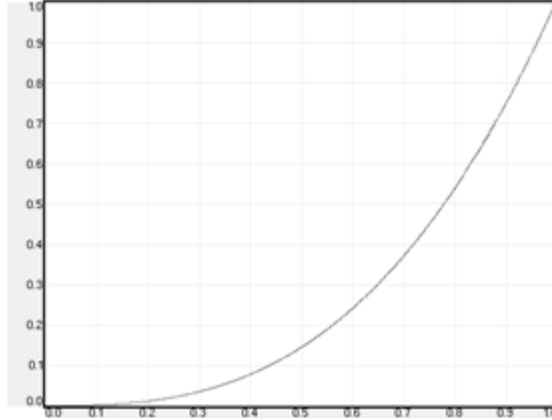
Figure 7-2. Film 2.8 gamma
