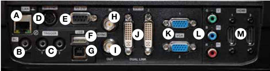
Figure 4-7. Connector panel
