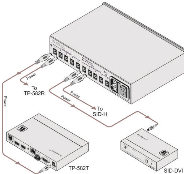
Figure 2: Connecting the VA-102P512 Power Supply
