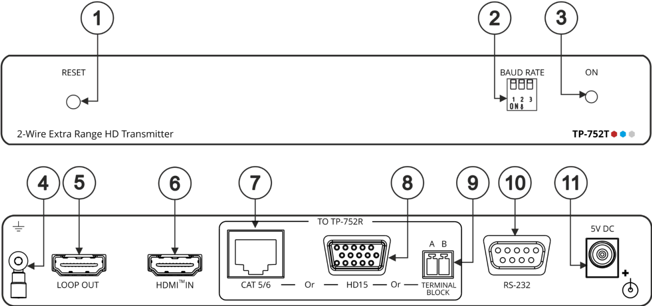
Figure 1: TP-752T 2-Wire Extra Range HD Transmitter
