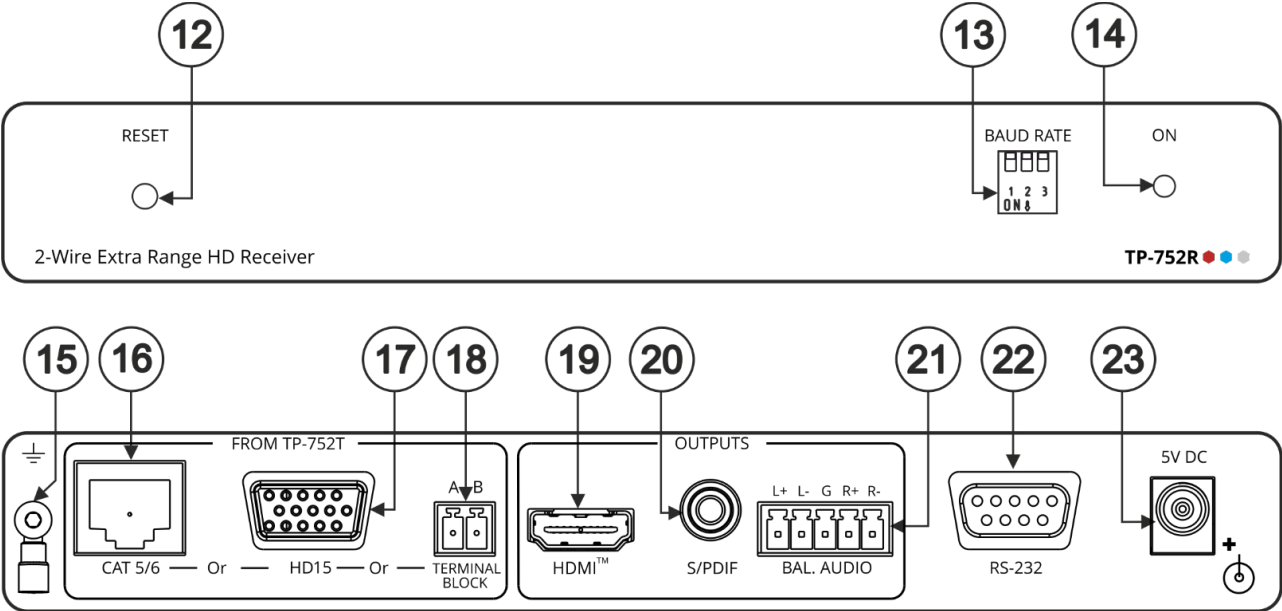
Figure 2: TP-752R 2-Wire Extra Range HD Receiver
