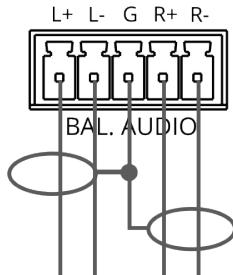
Figure 5: Connecting to a Balanced Stereo Audio Acceptor
