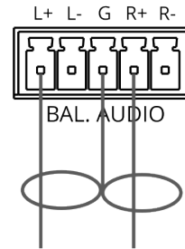
Figure 6: Connecting to an Unbalanced Stereo Audio Acceptor
