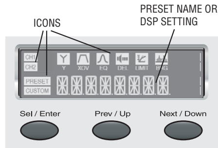
Figure 4.3 LCD Screen and Menu Navigation Buttons
