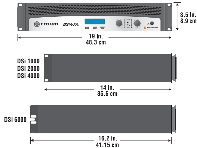
Figure 2.1 Dimensions
