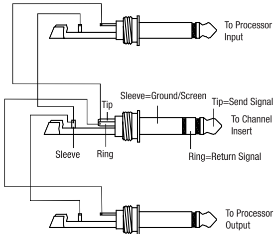
Y-Stereo lead for insert Connection
