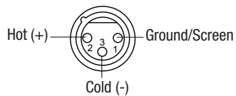
Use for Main output (For unbalanced use, leave pin 3 unconnected) 3-Pin XLR line socket (seen from soldering side)
