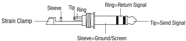
Use for Pre-Gain Channel Inserts 1/4" Stereo (TRS) Jack Plug
