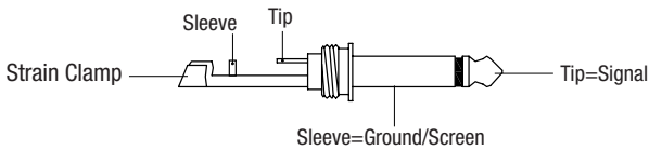
Use for Mono Line In, Mono 1/4" Jack Plugs 1/4" Mono (TS) Jack Plug
