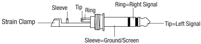
Use for Headphone, Stereo Return 1/4" Stereo (TRS) Jack Plug
