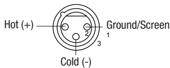
Use for Balanced Mic Inputs (For unbalanced use, connect pin 1 to 3) 3-pin XLR male plug (seen from soldering side)
