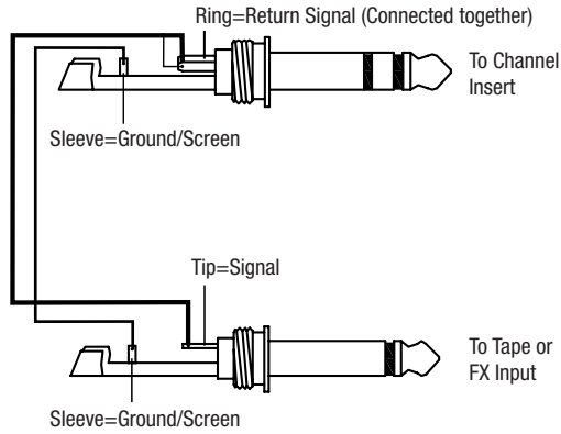
,Tapped' Connection Direct Output Lead (Enables the Insert to be used as a Direct Output while maintaining the channel signal flow)
