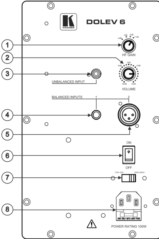
Figure 1: Dolev 6 Active 2-Way, Bi-Amplified Studio-Grade Speaker
