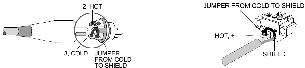
Illustration 2.11: Unbalanced connection of input
