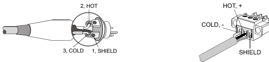
Illustration 2.10: Balanced connection of input
