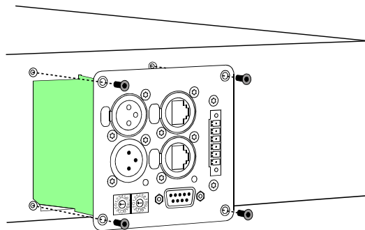
Illustration 4.1: Installation of a RCM-26
