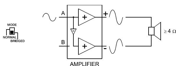
Illustration 2.9 : Mode BRIDGED
