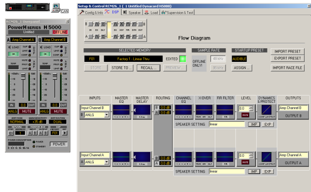
Illustration 4.3: DSP flow diagram of the RCM-26
