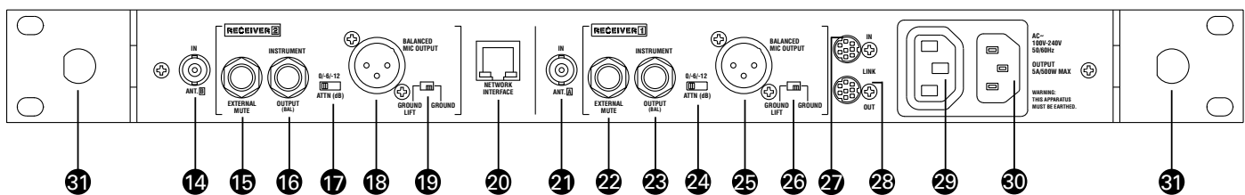
Fig. D AEW-R5200 Receiver Rear Panel
