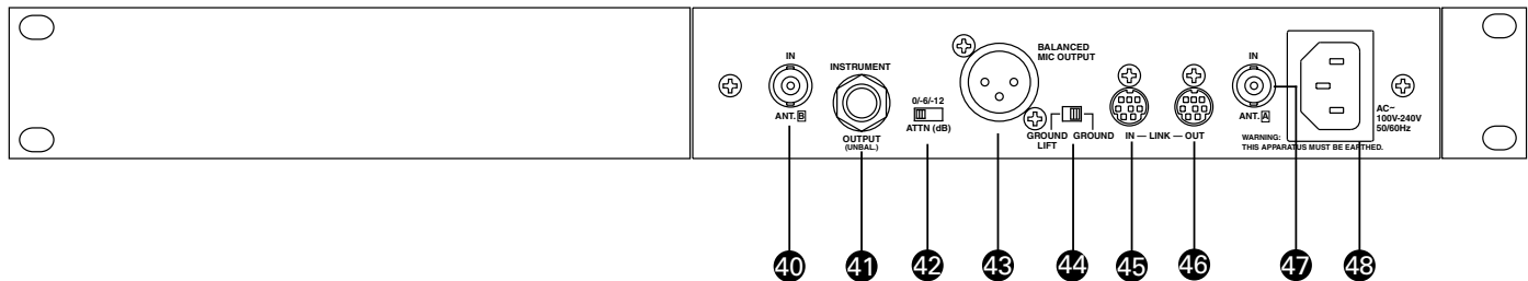
Fig. F AEW-R4100 Receiver Rear Panel
